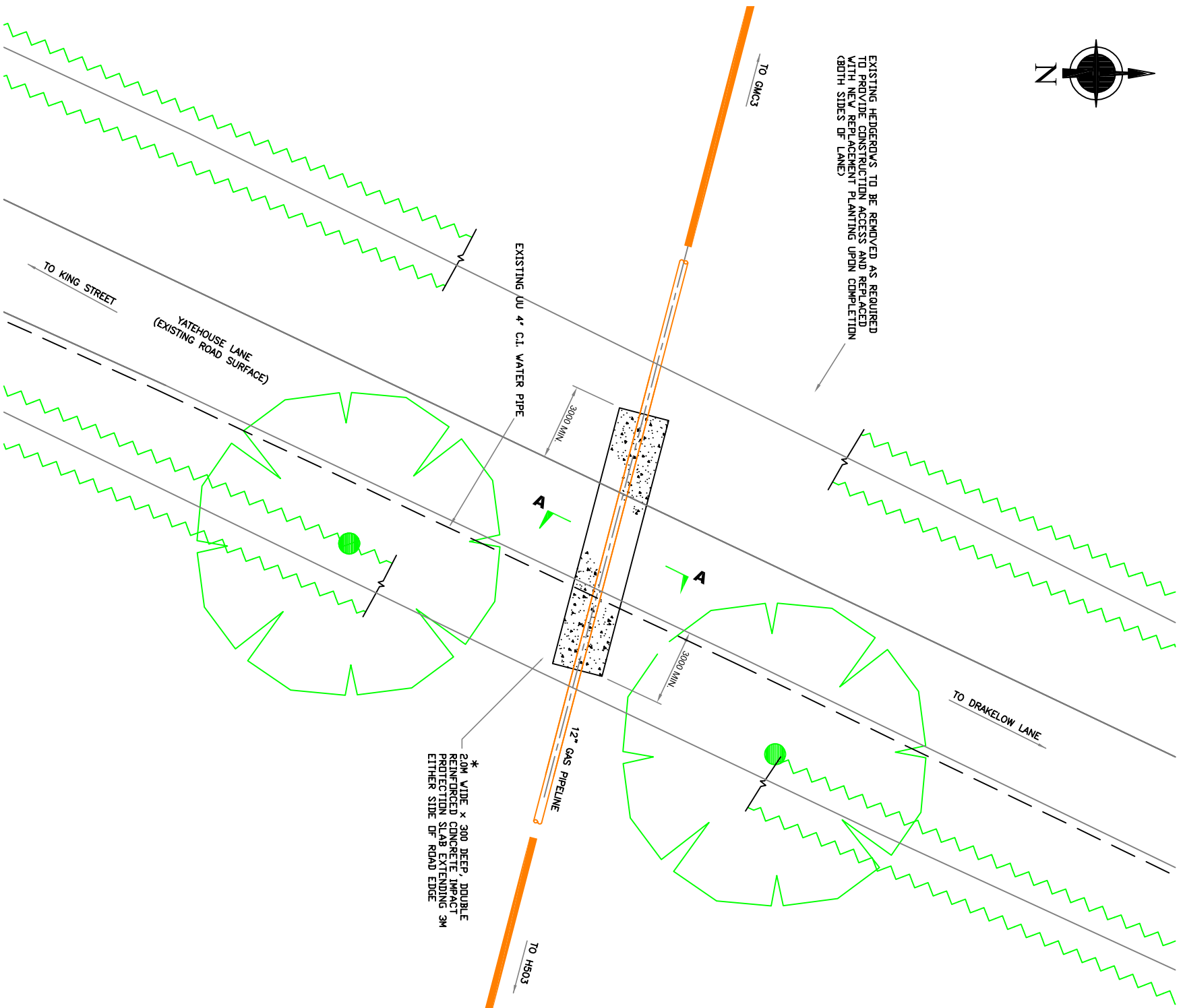
PLAN ON ROAD PIPELINE CROSSING YL1 1:200
